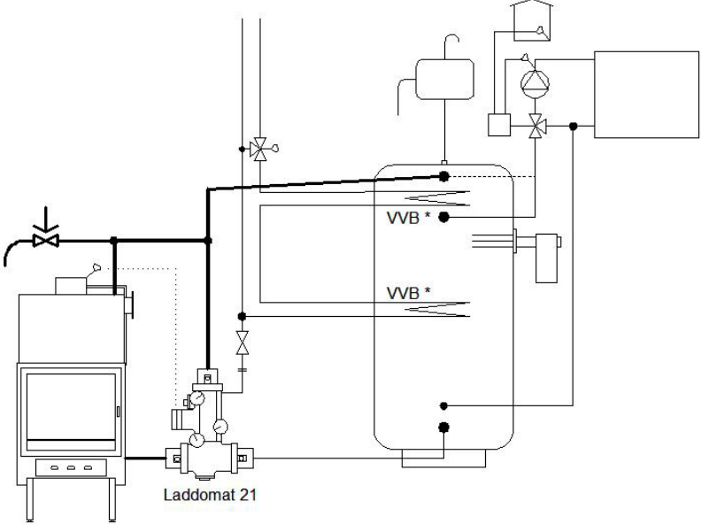
Schema 1: Stove with accumulation tank
