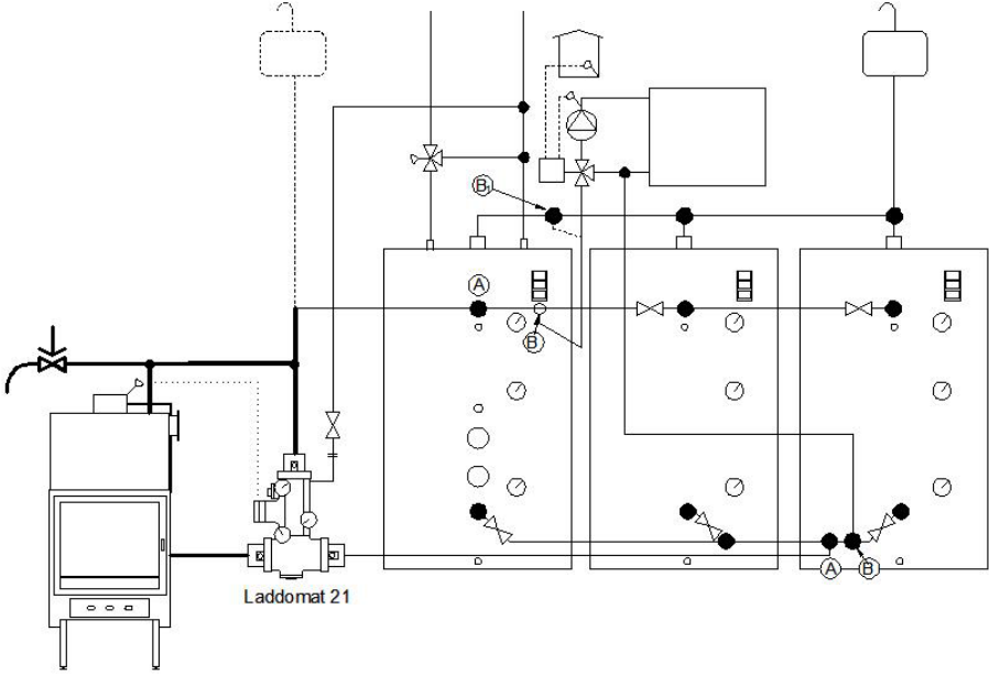
Schema 2: Stove with 3 accumulation tank
